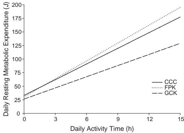
Fig. 2. Average daily resting metabolic expenditure of a 5-g S. graciosus is shown for each of the three study populations for activity periods of up to 15 h. As the duration of activity increases, lizards from CCC and FPK incur higher energetic costs than do lizards from GCK.
