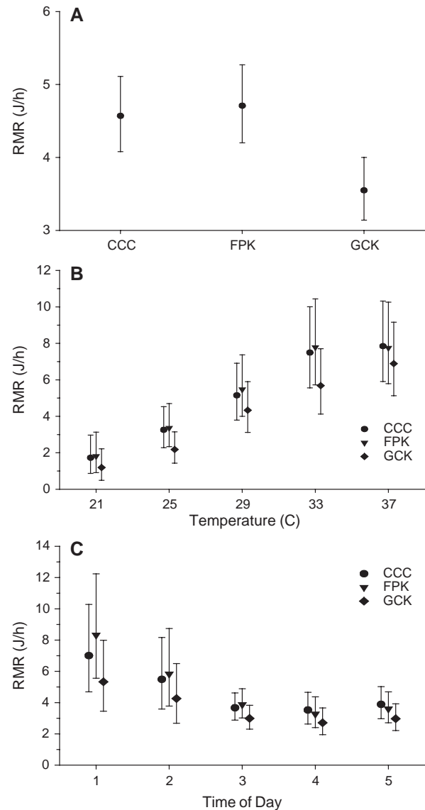
Fig. 1. Lizards from GCK exhibited lower RMR than did lizards from CCC or FPK. RMR is plotted with respect to (A) study population, (B) body temperature, and (C) time of day that metabolic rates were measured. In each graph, least square means (LSM) are plotted along with 95% confidence intervals, and all plotted values have been untransformed (from log values) from the analysis. For viewing clarity, the plotted values of metabolism for each population are offset at each temperature and time of day.
